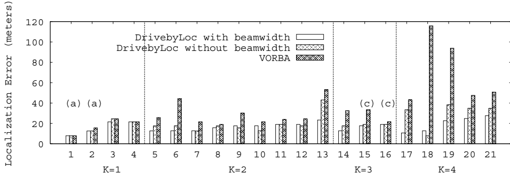
Fig. 8. Comparison of DrivebyLoc and VORBA.
